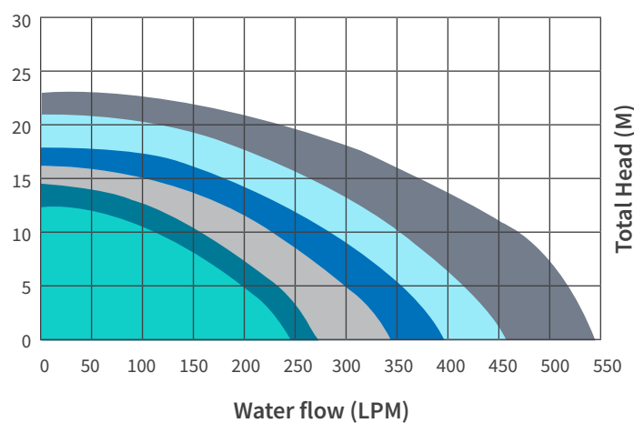
PR Series Performance Curves
