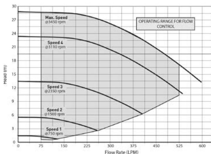
Performance Curves
