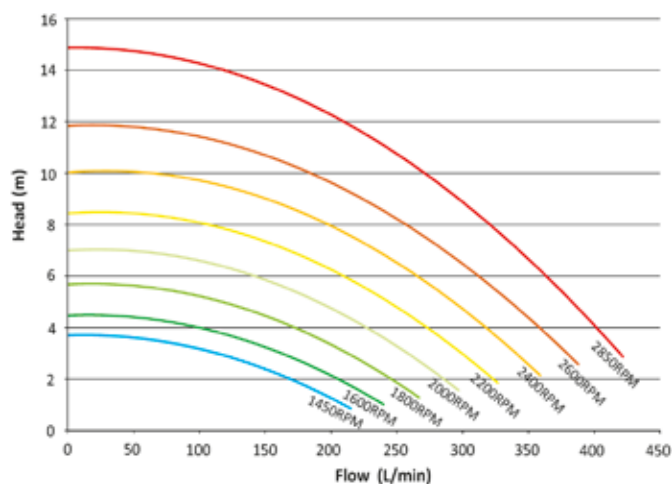
EnviroMAX 800 Performance Chart
