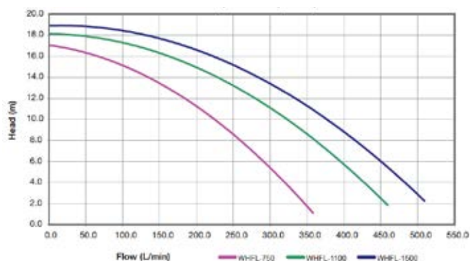
Whisperflow Pump Family Performance Chart
