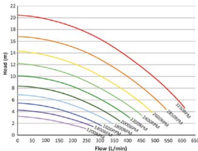
EnviroMAX 1500 Performance Chart
