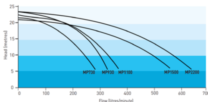
Max-e Pro Performance Chart
